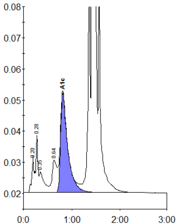
Peak table - ID: 10435809
